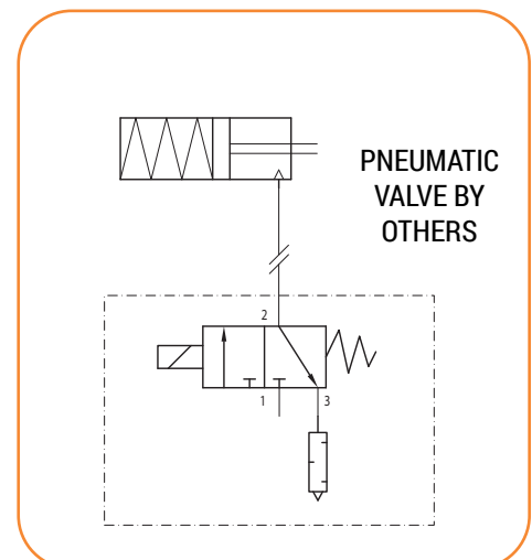
PNEUMATIC SCHEMATIC
