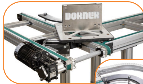
90 Degree Corner
