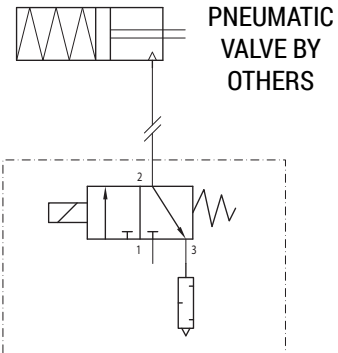
PNEUMATIC SCHEMATIC
