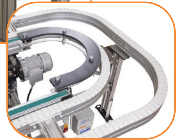
180 Degree Corner
