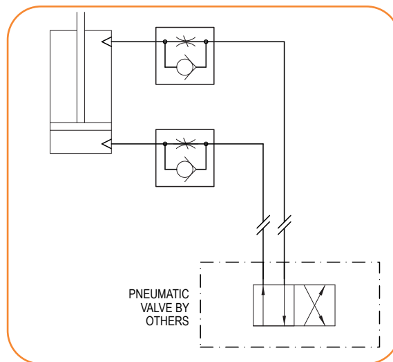
PNEUMATIC SCHEMATIC
