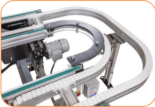
180° Corner
