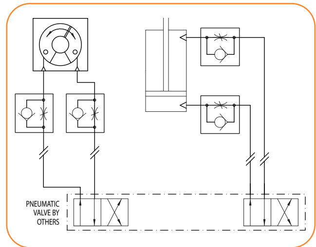
PNEUMATIC SCHEMATIC
