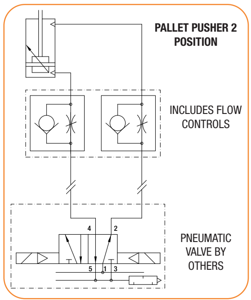
PNEUMATIC SCHEMATICS
